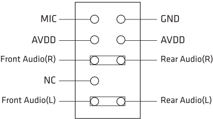
Exp. MB pins-layout
